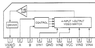
IC21, 24, 25 : LA7956 Video Switch
