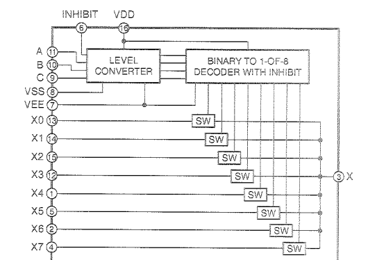
IC602 : HD74HC4051P Analog Multiplexers/Demultiplexers
