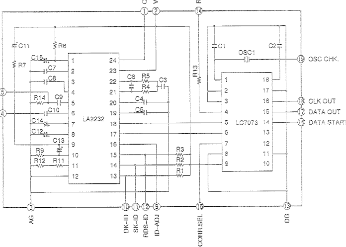
RDS Decoder & Controller
