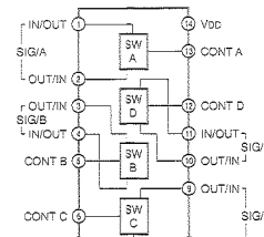
IC29 : μPD4068BC Quad Analog Switch/Multiplexer
