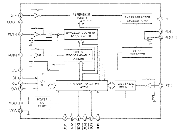
PLL Controller
