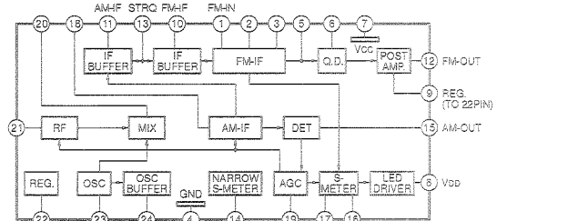
AM/FM IF
