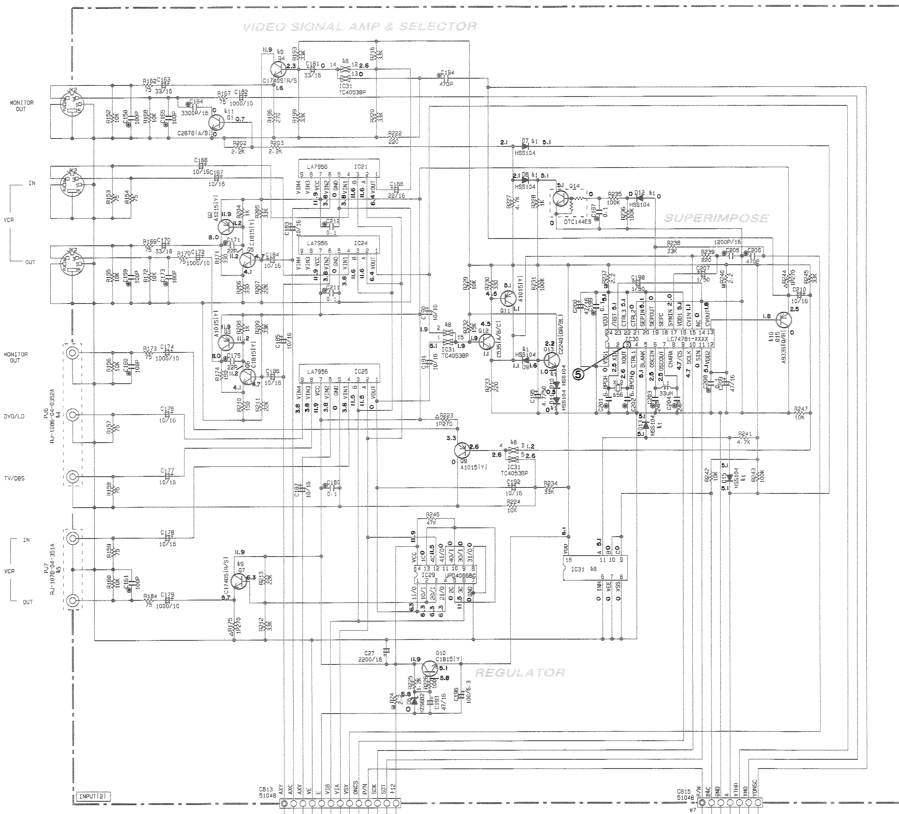
IC21, 24, 25 : LA7956 Video Switch
