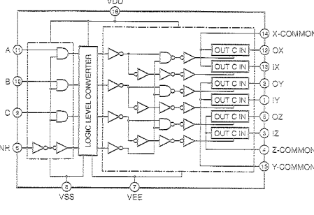
IC31 : TC4068BP Triple 2-Channel Multiplexer/Demultiplexer
