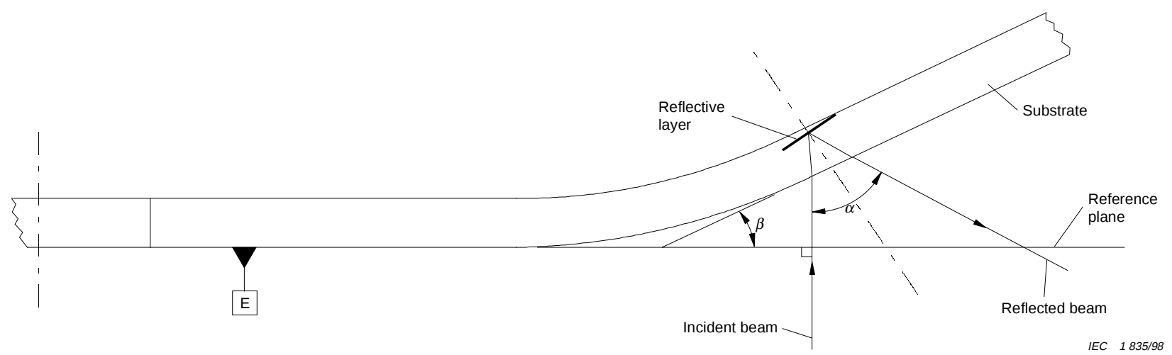
Figure 16 – Angular deviation
