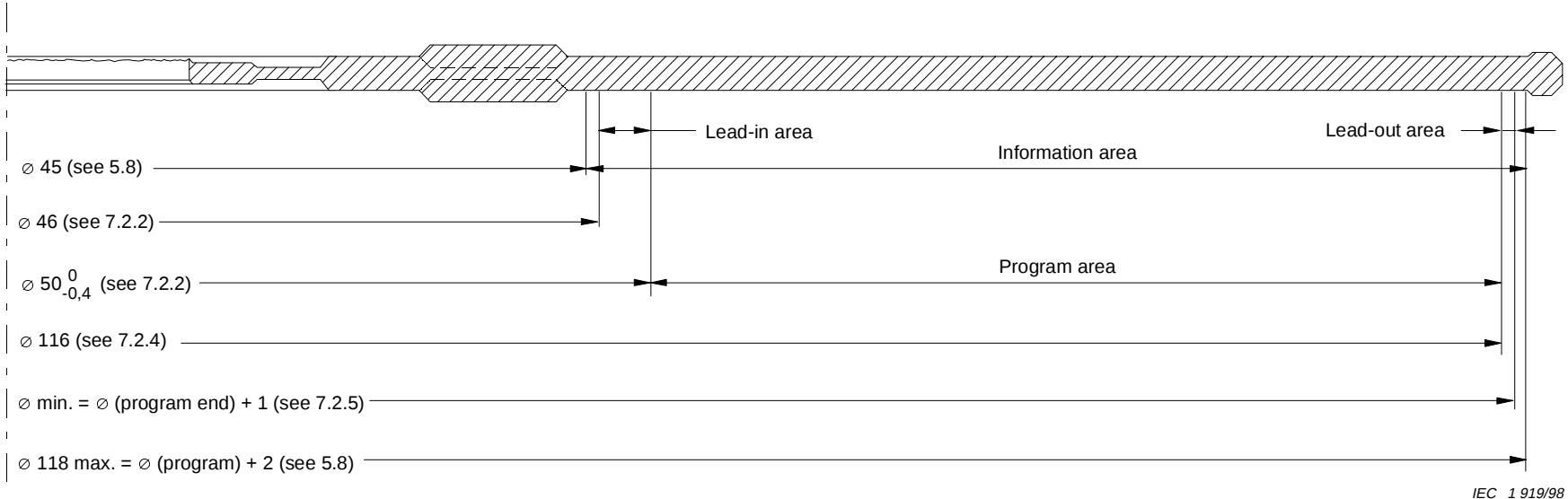
Figure 2c – Dimensions of the disc
