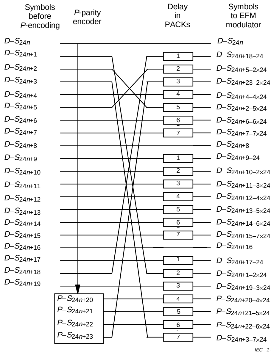
Figure 21 – P-parity and interleave sequence
