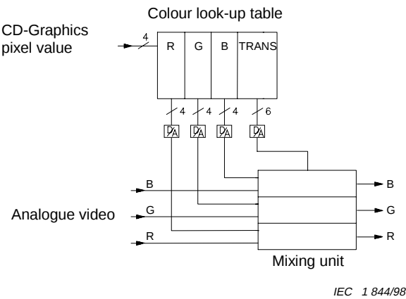
Figure 25 – Block diagram of a video/graphics mixing unit
