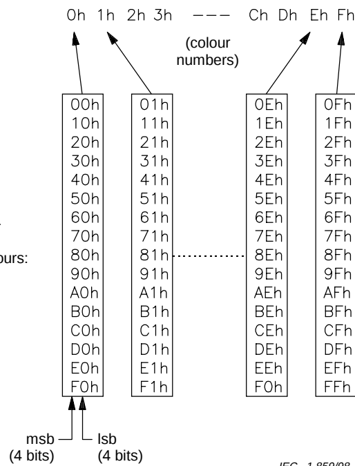
Figure F.3 – Relationship of colours between TV-Graphics and EXTENDED TV-Graphics
