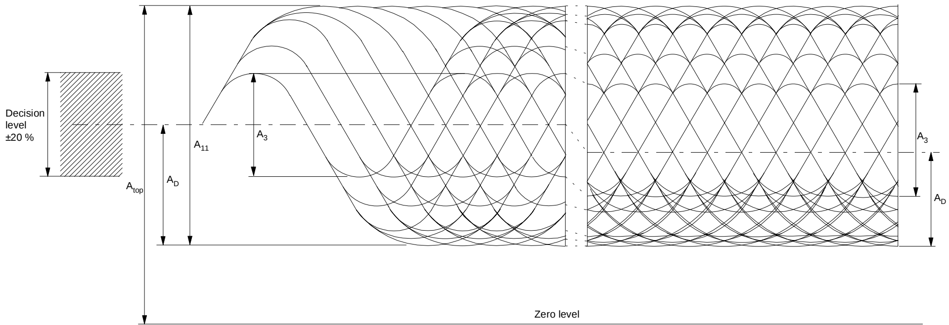
Figure 3 – HF signal
