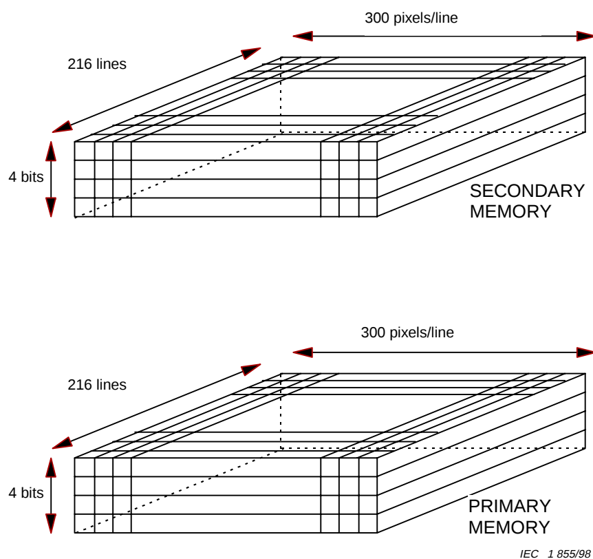
Figure F.1a – Two memory planes of 16 colours
