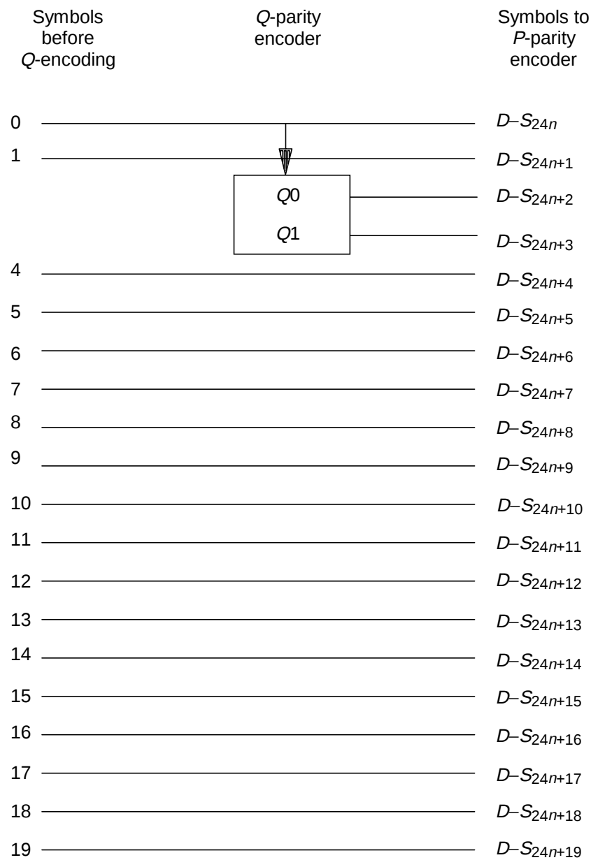
Figure 23 – Q-parity encoder
