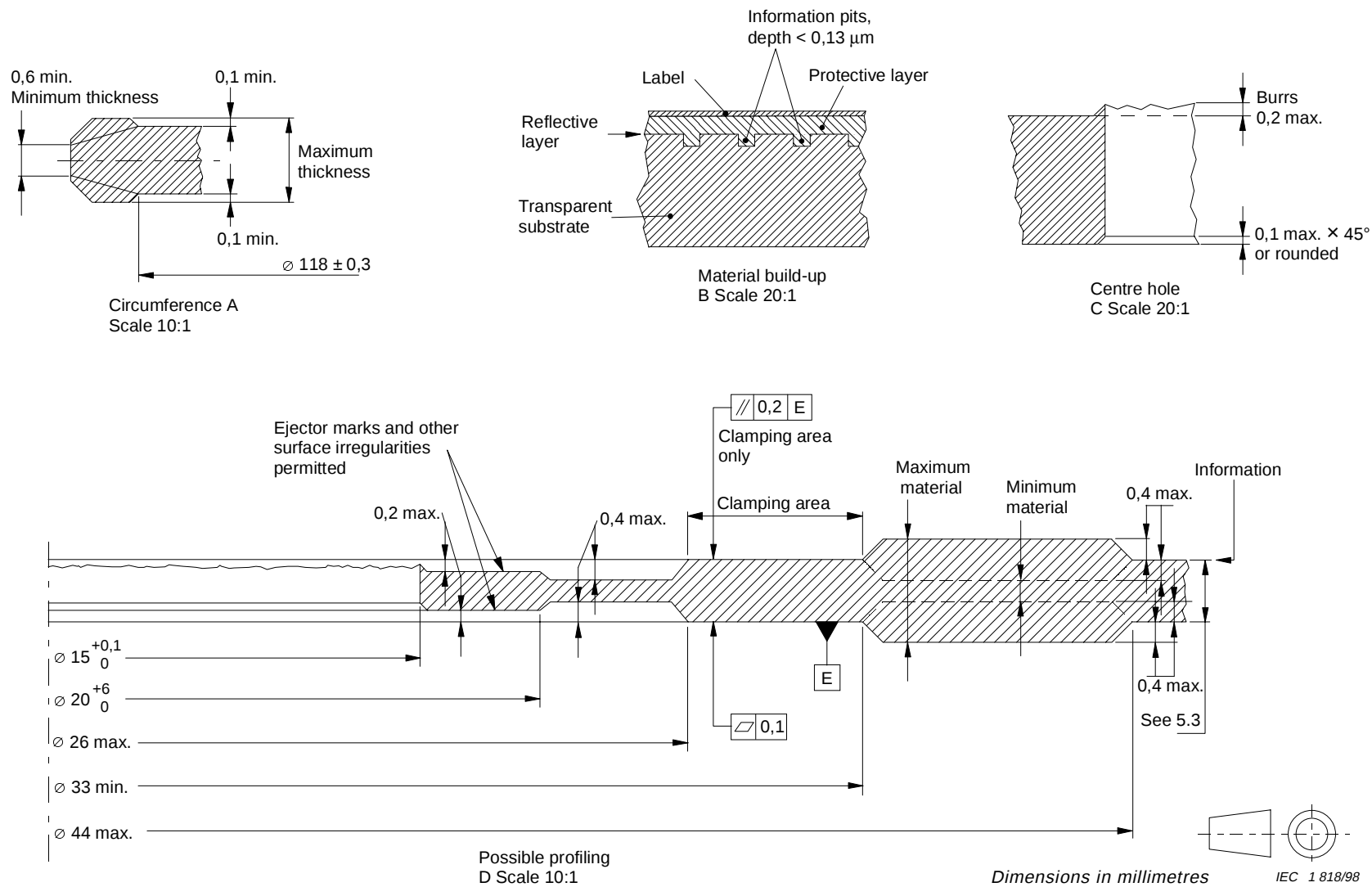
Figure 2b – Dimensions of the disc
