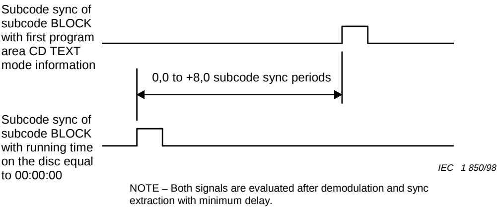
Figure 31 – Maximum allowed mode transition skew
