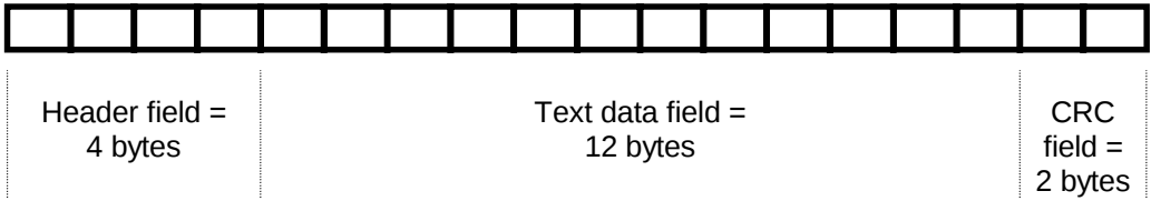
Figure 28 – CD TEXT mode PACK format for the lead-in area
