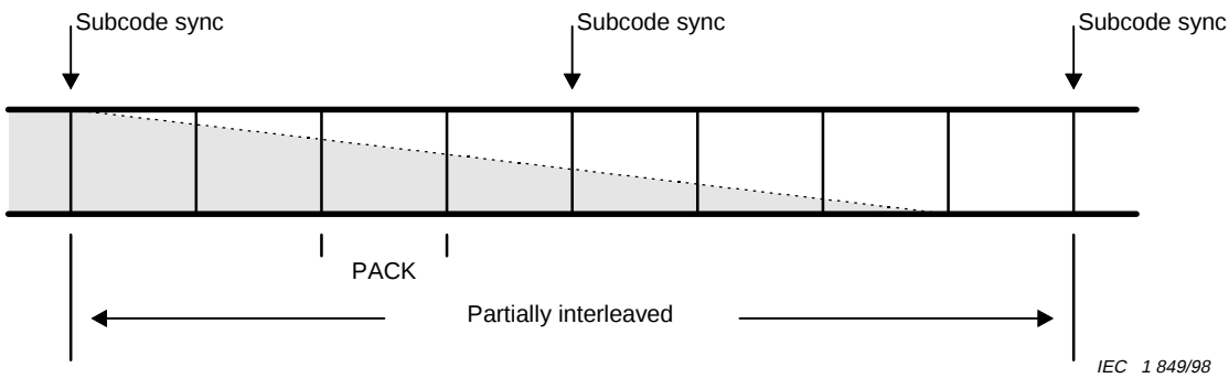
Figure 30 – Example of partial interleaving of PACKs
