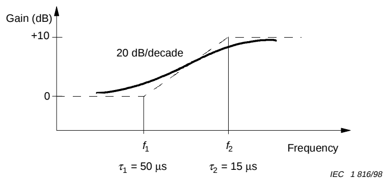
Figure 1 – Pre-emphasis characteristic
