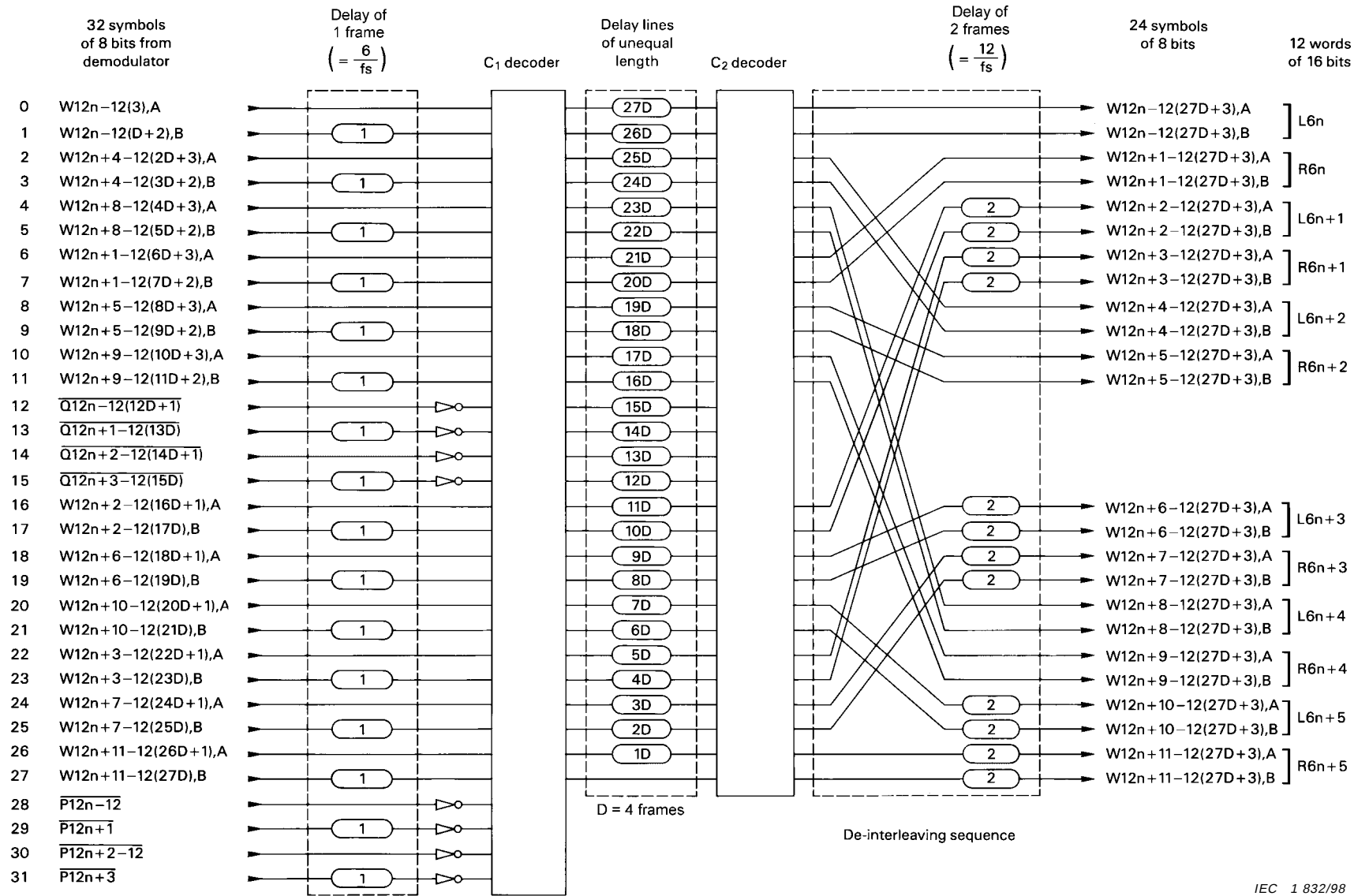
Figure 13 – CIRC decoder
