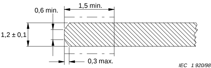
Figure 2d – Edge shape of the disc (8 cm-CD)
