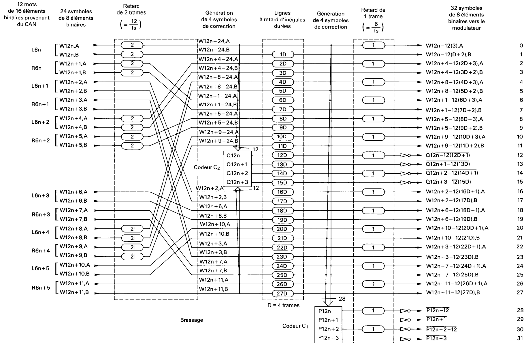
Figure 12 – Codeur CIRC
